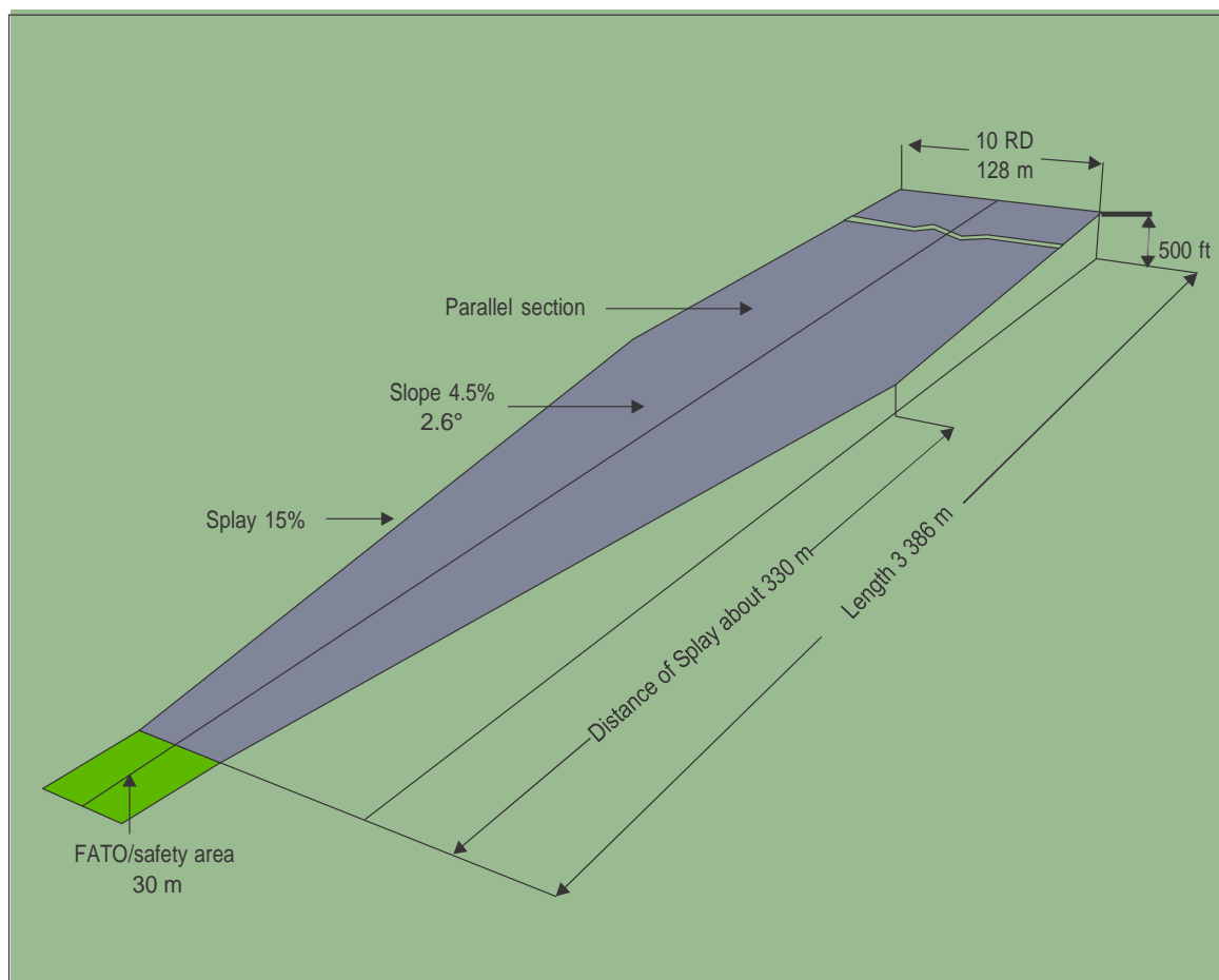
Figure II-4-16. Night category A slope (15 m D-value)
