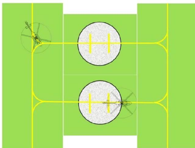
Figure II-3-19. Air taxi-through stands (with air taxi-route)
