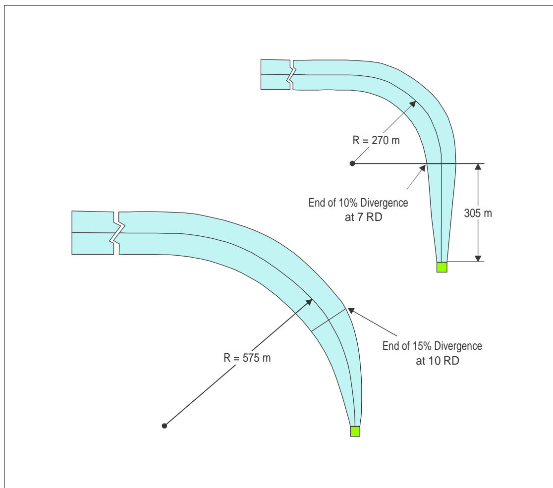
Figure II-4-1. Curved approach and take-off climb surface for all FATOs
