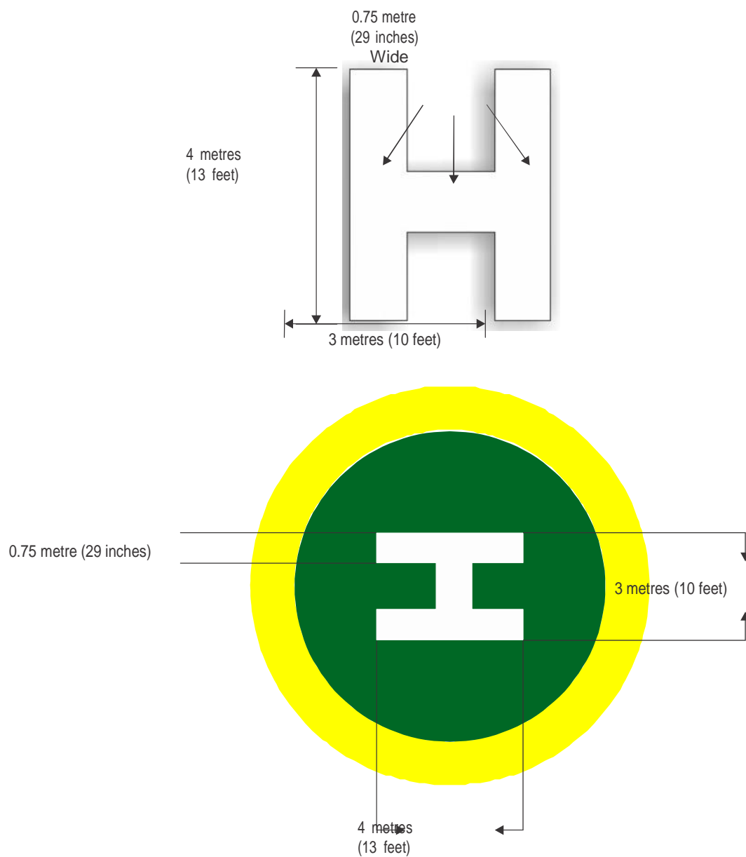
Figure I-5-2. Dimensions of the heliport identification “H” marking (standard size)
