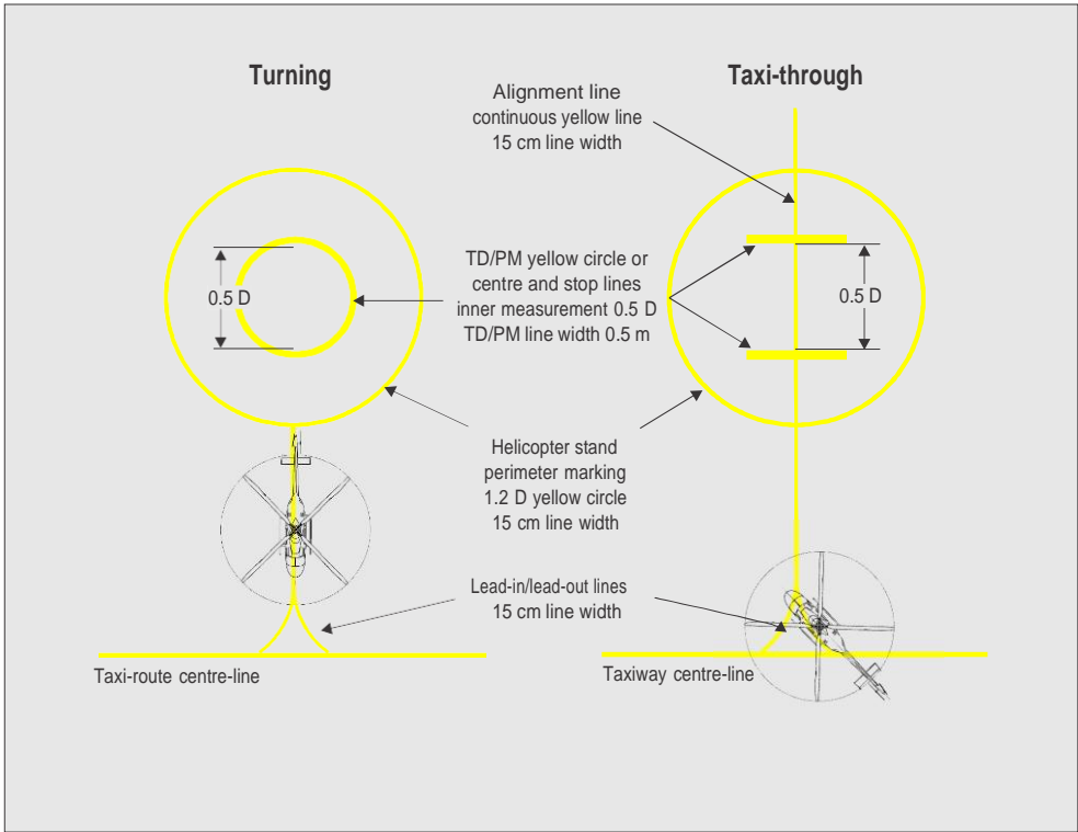
Figure II-5-18. Stand markings
