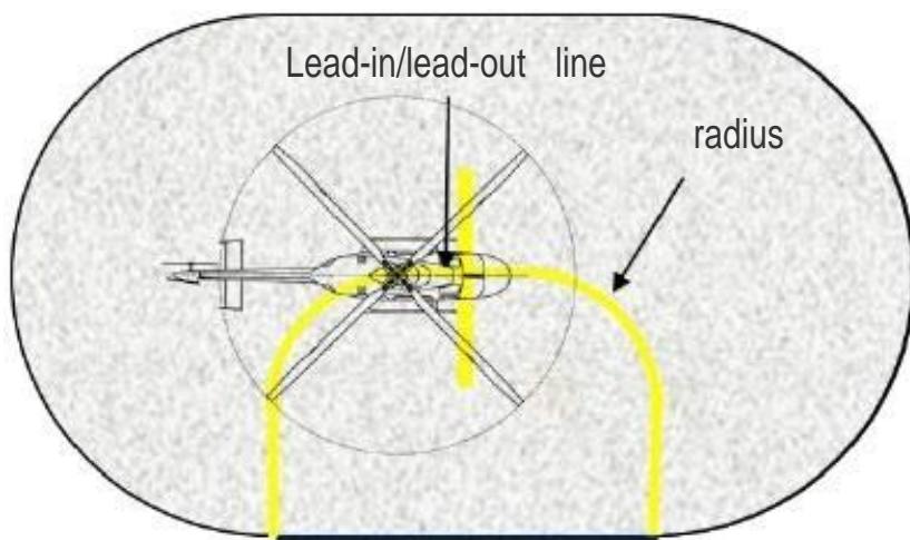
Figure II-3-15. Bi-directional ground-taxi stand with entry/exit from one side
