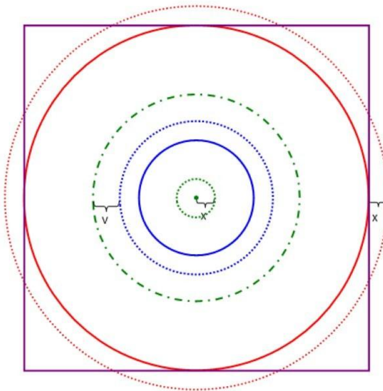
Figure II-3-C-1. Performance Class 1 TLOF/FATO (RTODR) dimensions
