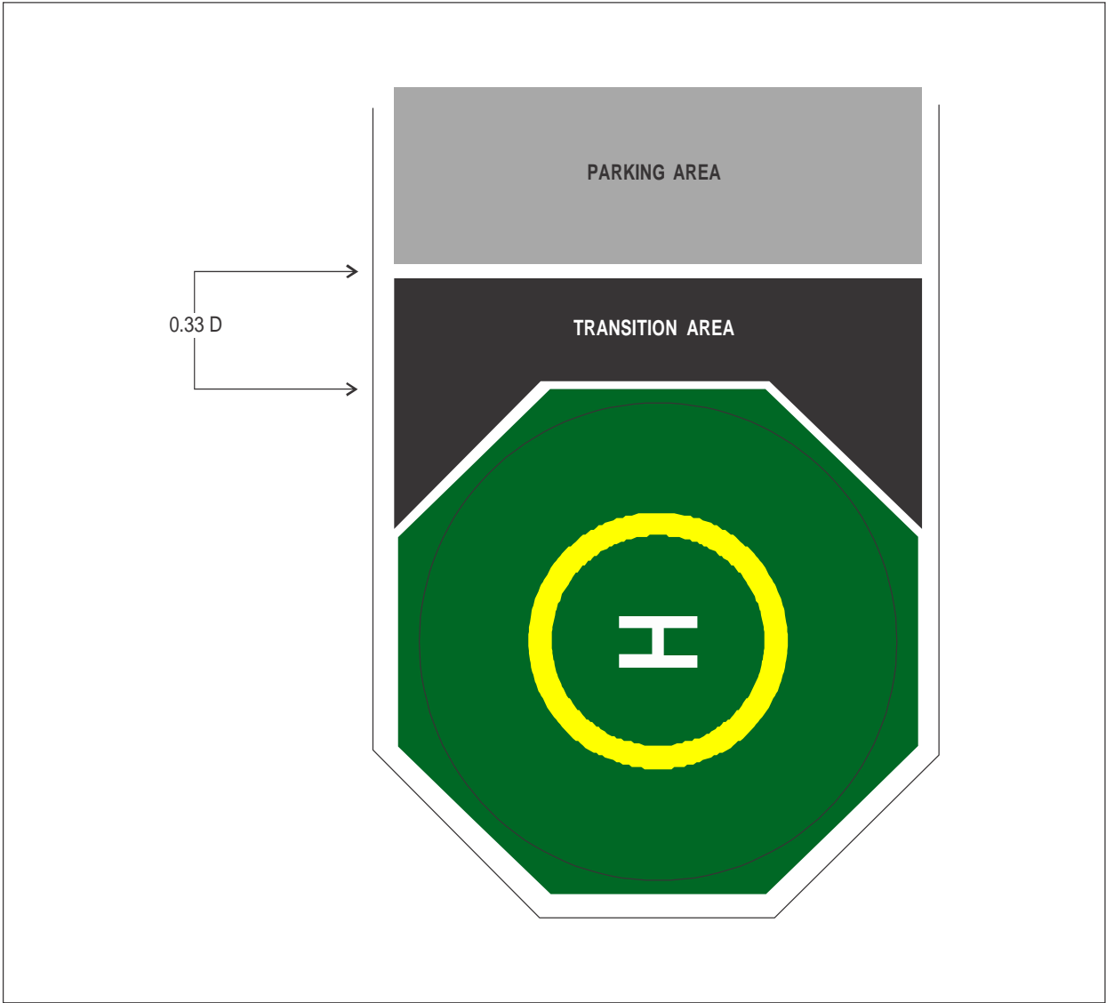
Figure I-8-4. Parking transition area (PTA)
