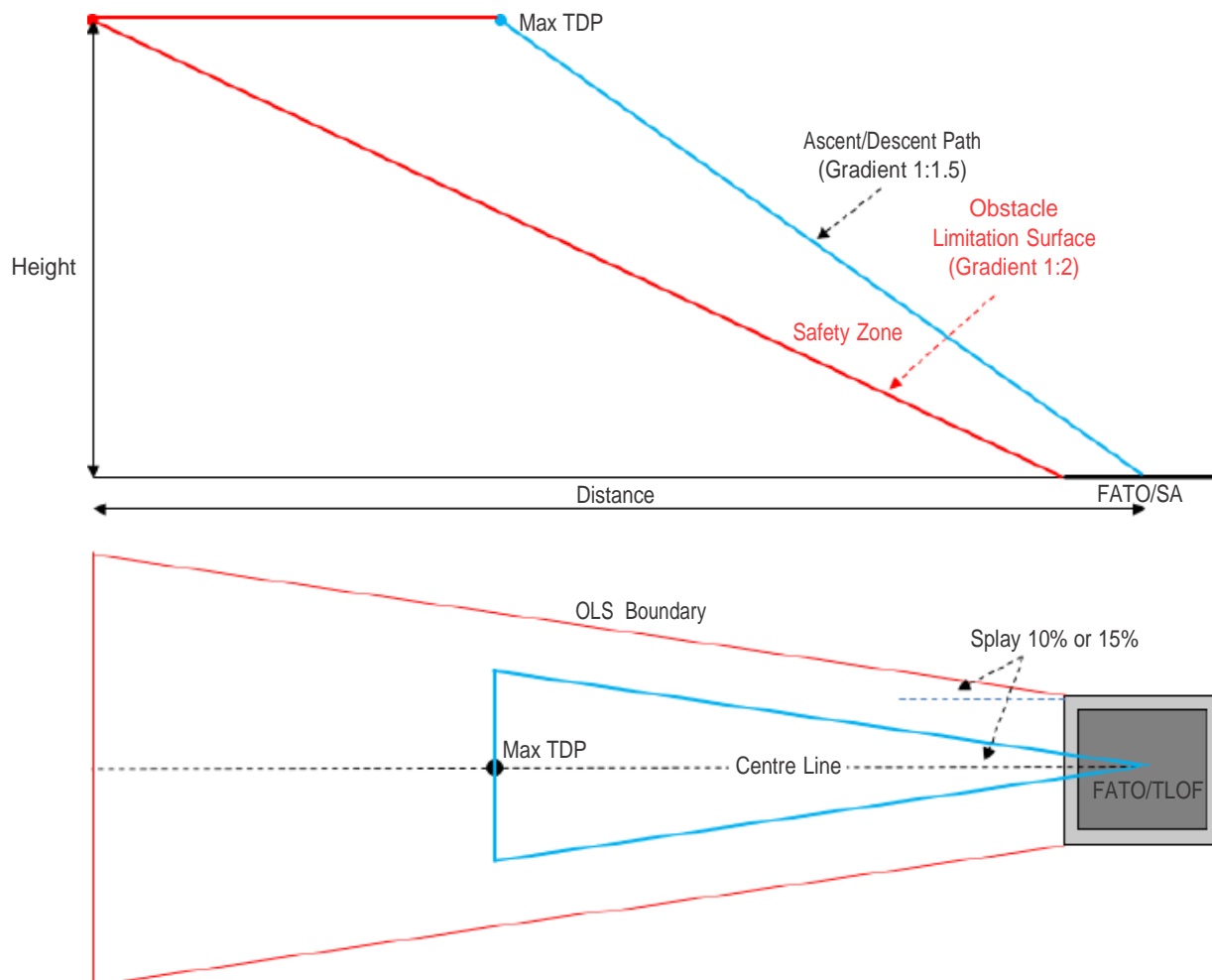
Figure II-3-10. Back-up area
