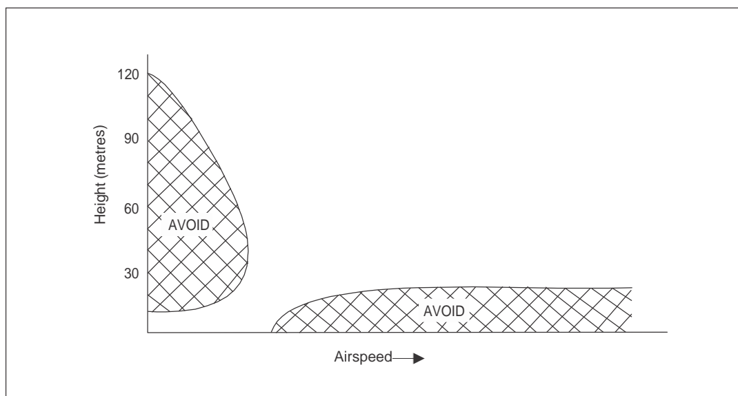
Figure II-2-1. HV Diagram
