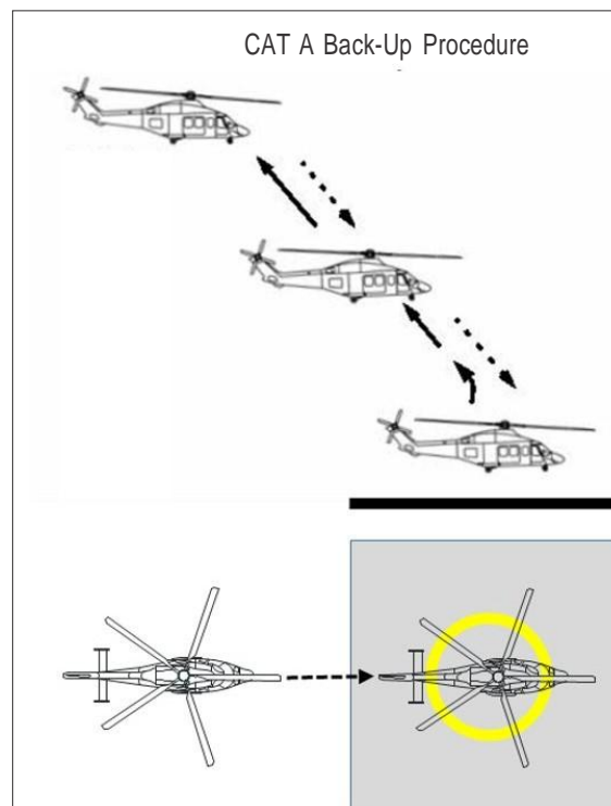
Figure II-3-5. PC1 (helipad) FATO without a declared RTODRH 15
