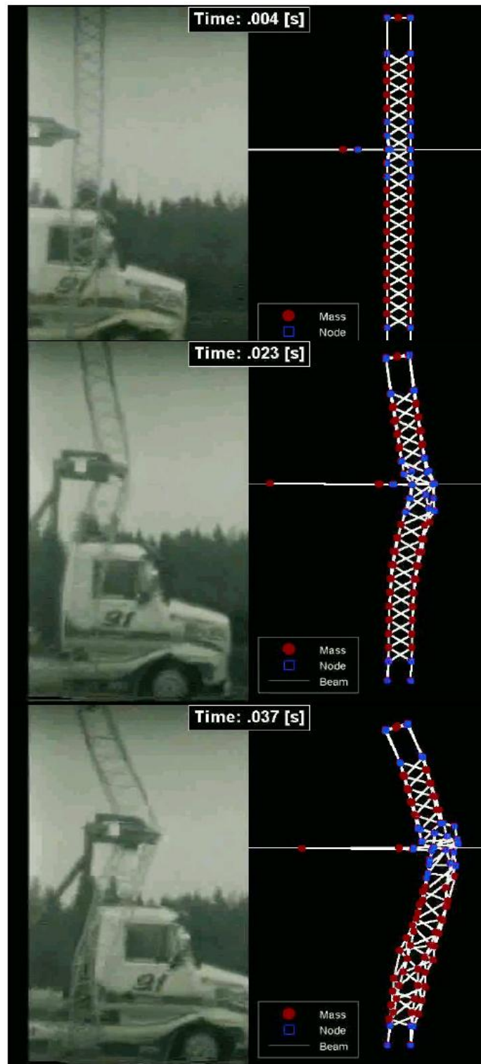
Figure 6-6. Comparison between actual deformation and that resulting from the hybrid analysis
