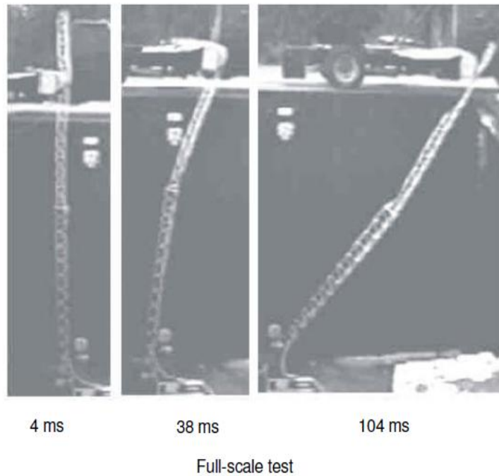
Figure 6-3. Impact events from finite element analysis (FEA) simulation and full-scale test — impact speed 140 km/h; impact on apex; top mass 5.44 kg; rigid impactor
