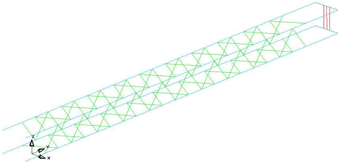
(a) Approach lighting tower — fiberglass lattice structure
