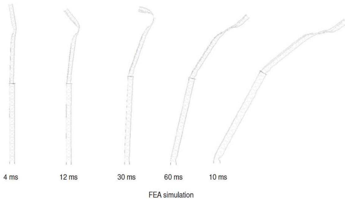
Figure 6-1. Examples of three-dimensional finite element analysis (FEA) Models of approach lighting towers
