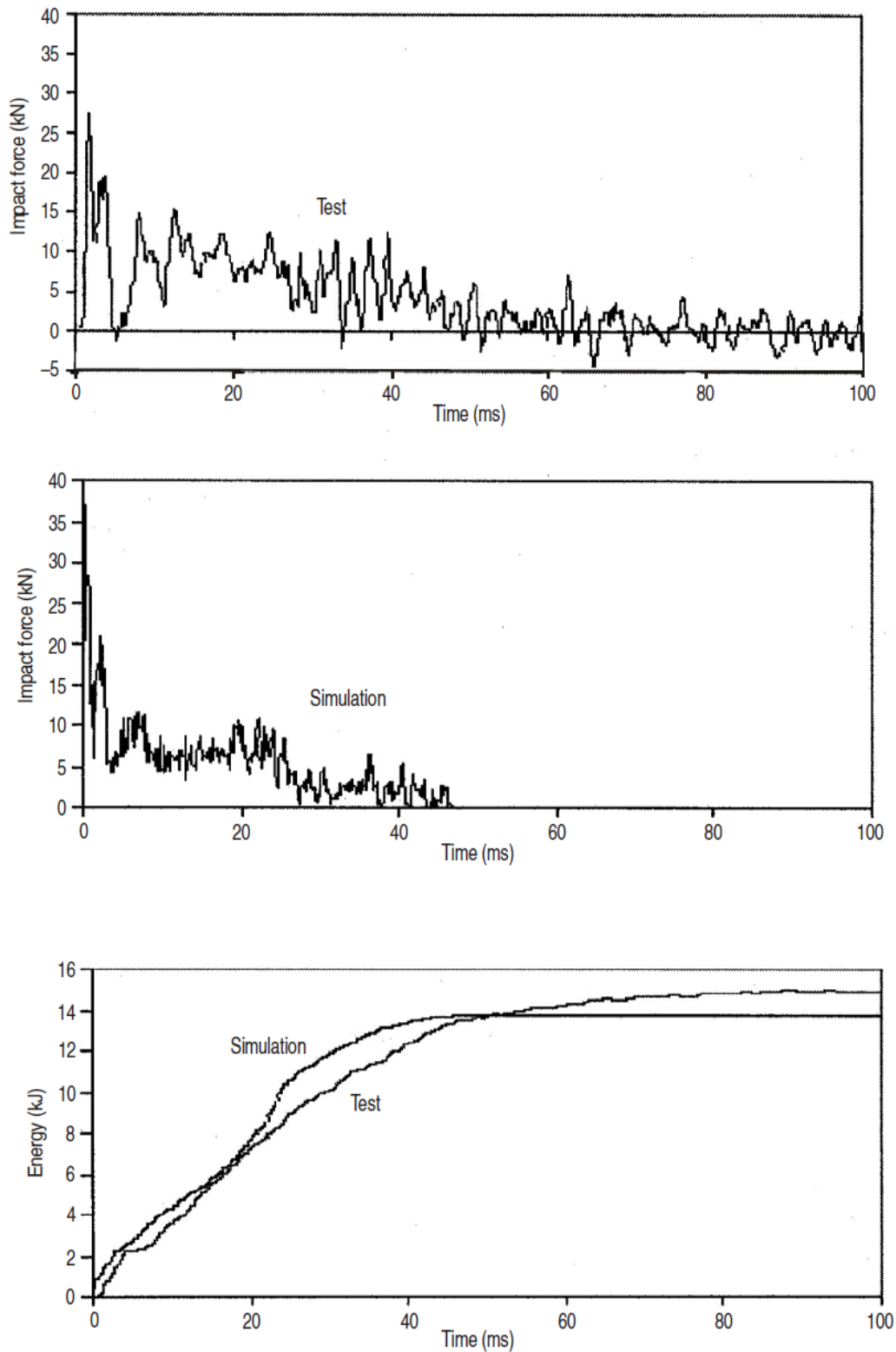
Figure 6-4. Impact force and energy — impact speed 140 km/h; impact on side; rigid impactor
