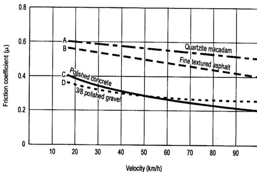
Figure 1-4. Relationship between braking friction coefficient achieved with anti-skid braking on different textured surfaces at certain operating conditions
