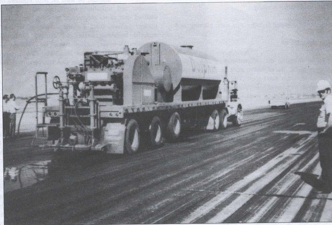
Figure 8-1. Oscillating high-pressure water vehicle
