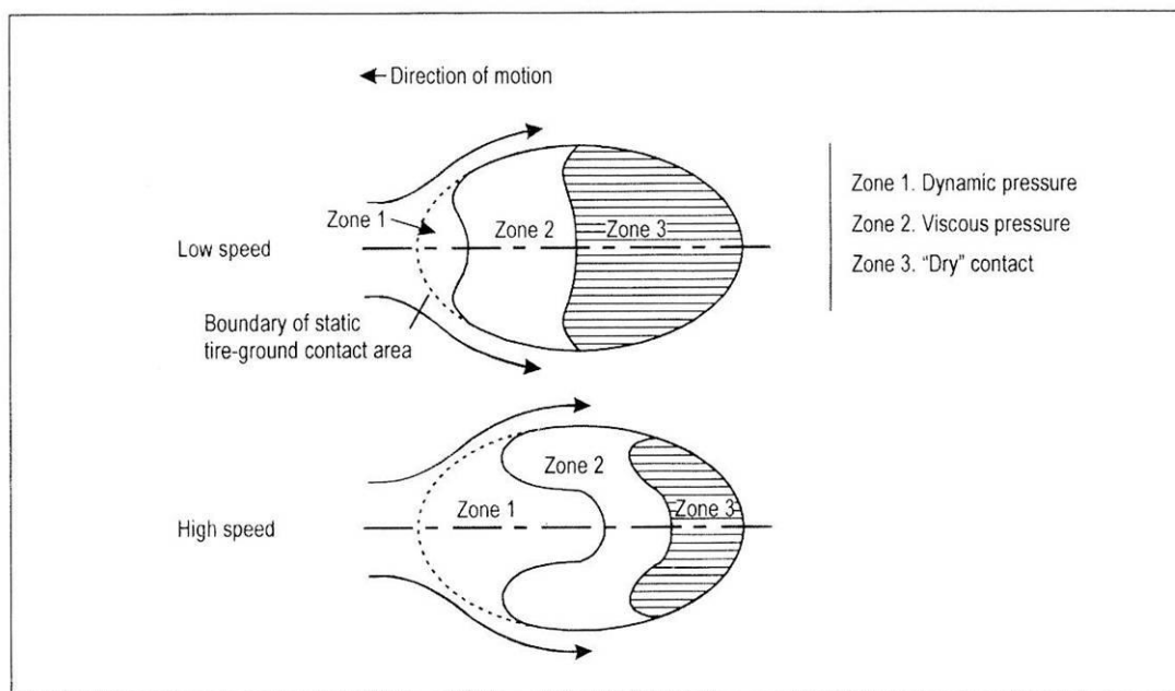
Figure 1-3. Areas of tire/surface interface
