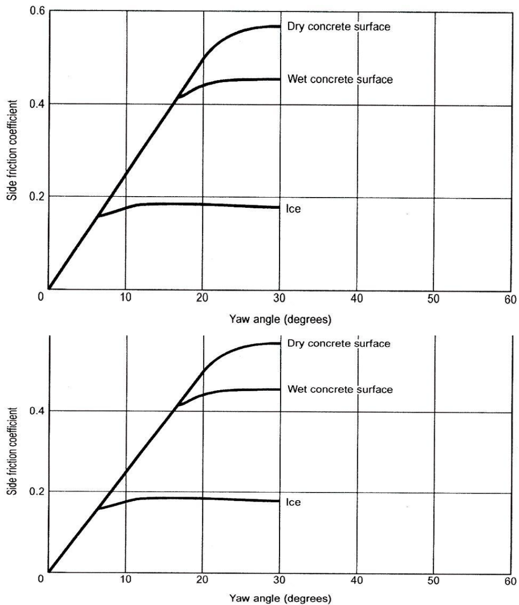
Figure 1-2. Typical variation of side friction coefficient with yaw angle
