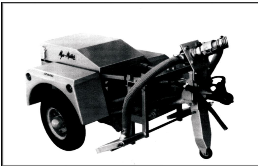
Figure 5-4. Mu-meter trailer
