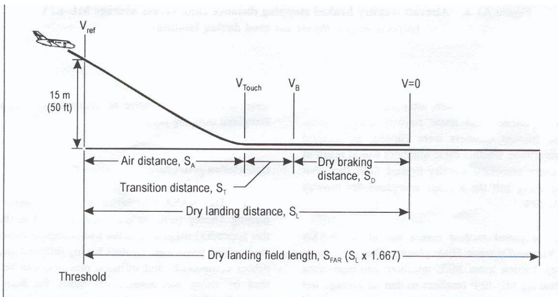
Figure A1-1. Aircraft landing terminology
