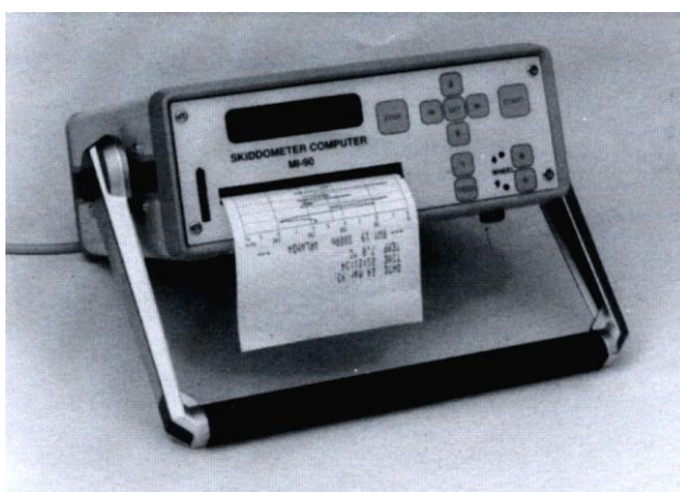
Figure 5-9. MI-90 computer for Skiddometer BV-11 trailer
