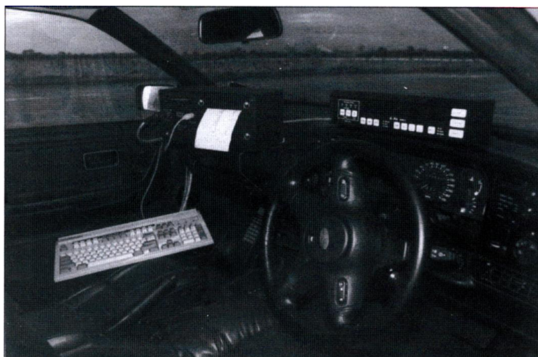
Figure 5-5. Processor unit and keyboard for Mu-meter trailer
